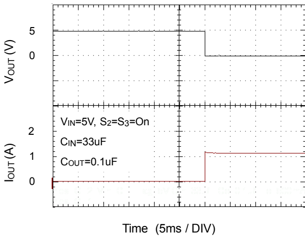
Short Circuit Current Response ⑤
