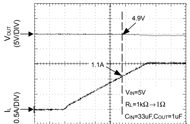
Ramped Load Response ⑤
