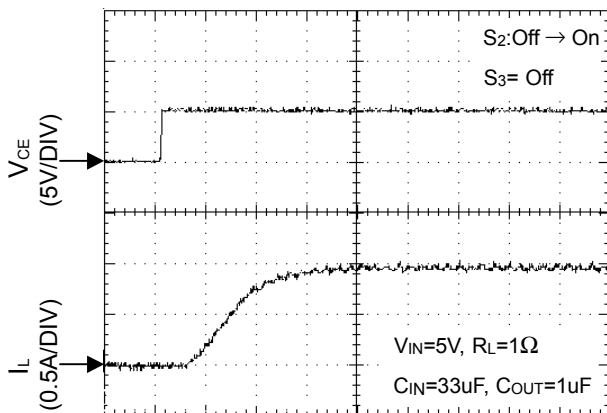
Soft-Start Response ⑤
