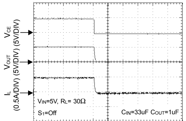
Turn-Off Response ①
