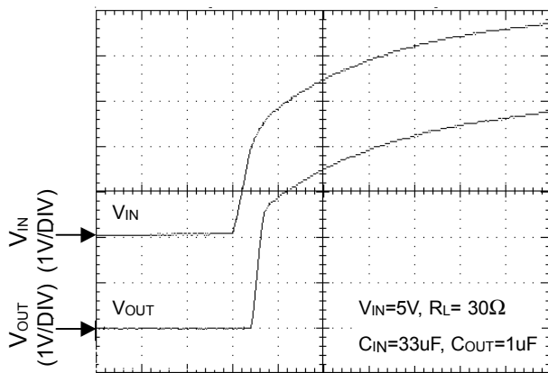
UVLO at Rising ④
