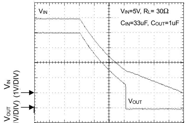
UVLO at Falling ④
