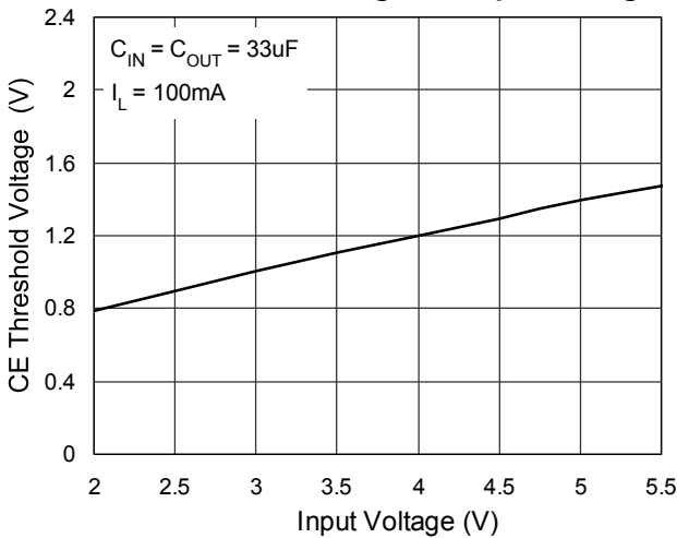
CE Threshold Voltage vs. Input Voltage ④
