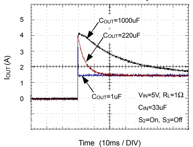
Short Circuit Current Response
