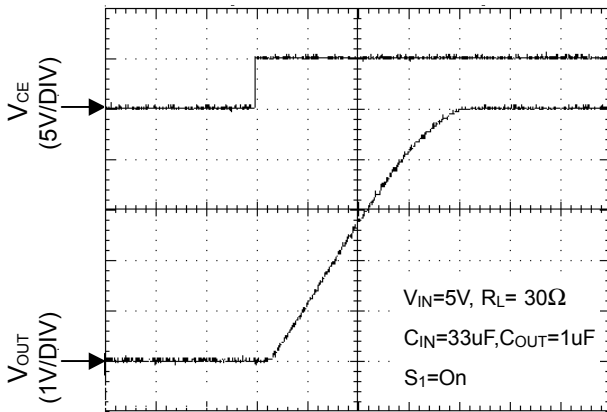
Turn-On Response ①
