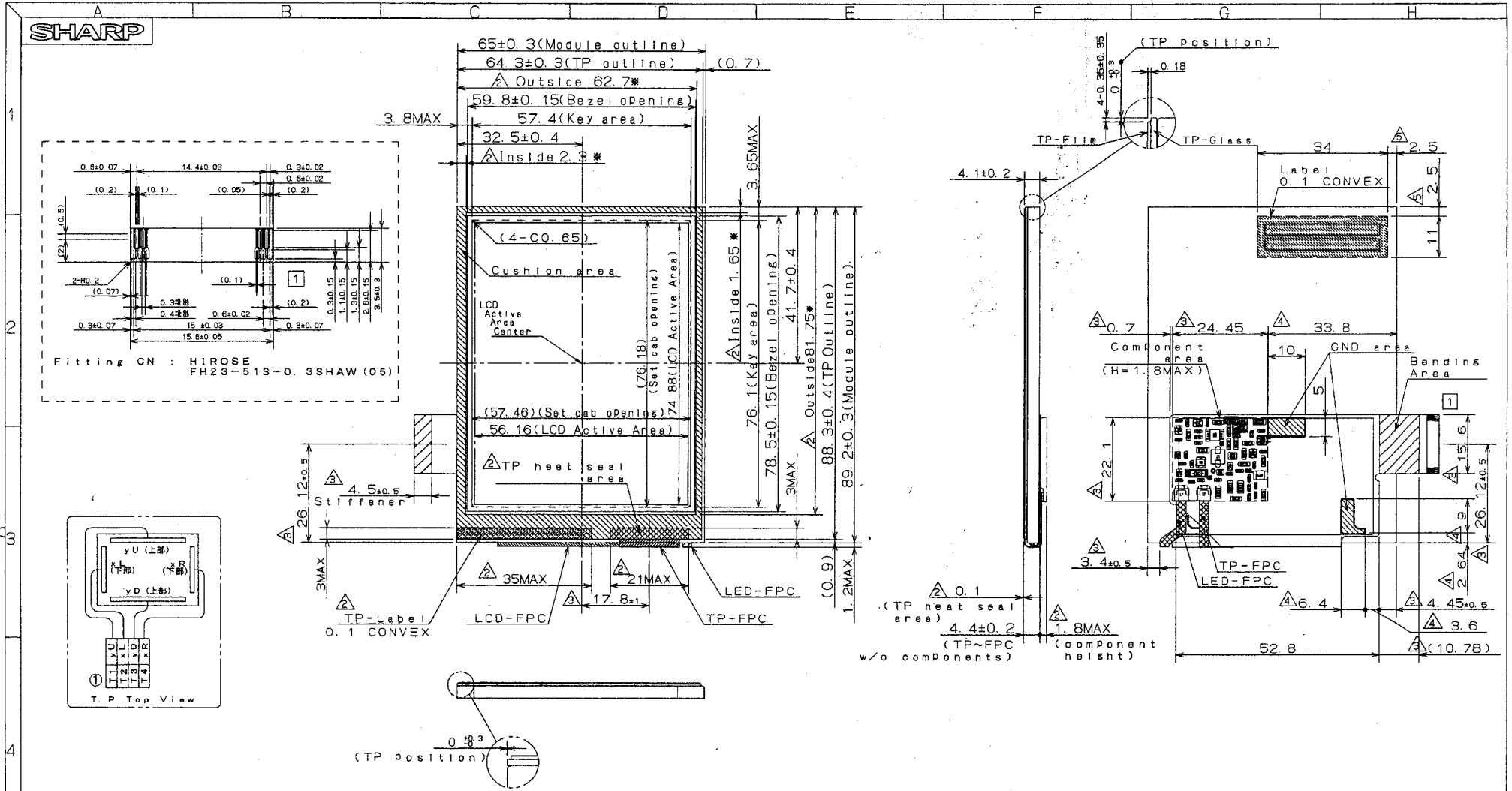
Fig. 1 Outline dimensions
